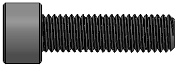
M10-1.5 X 35mm HEX HEAD BOLT - 12.9 920-0119 (1)
